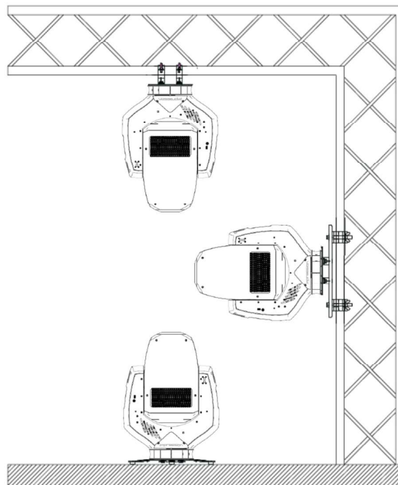
Figure 5. Mounting Options
