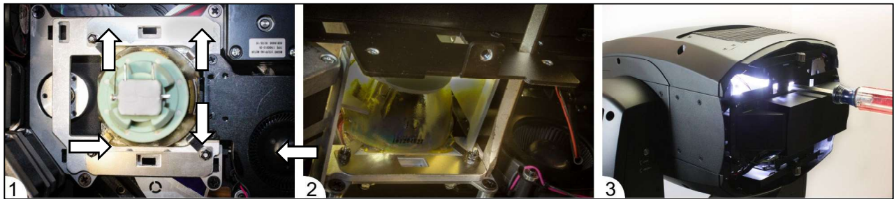
Figure 20: Lamp adjustment
