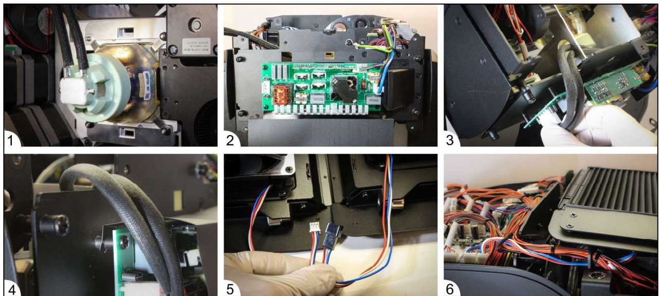
Figure 19: Lamp installation
