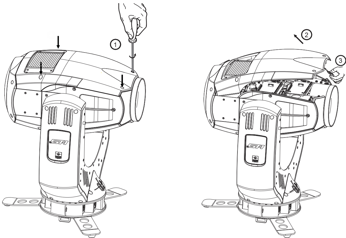
Figure 13. Head cover removal
