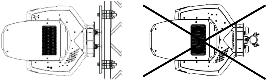
Figure 9. Sideways Mounting
