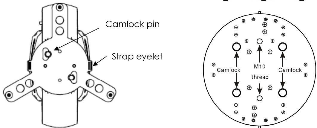
Figure 6. Upright Mounting Details
