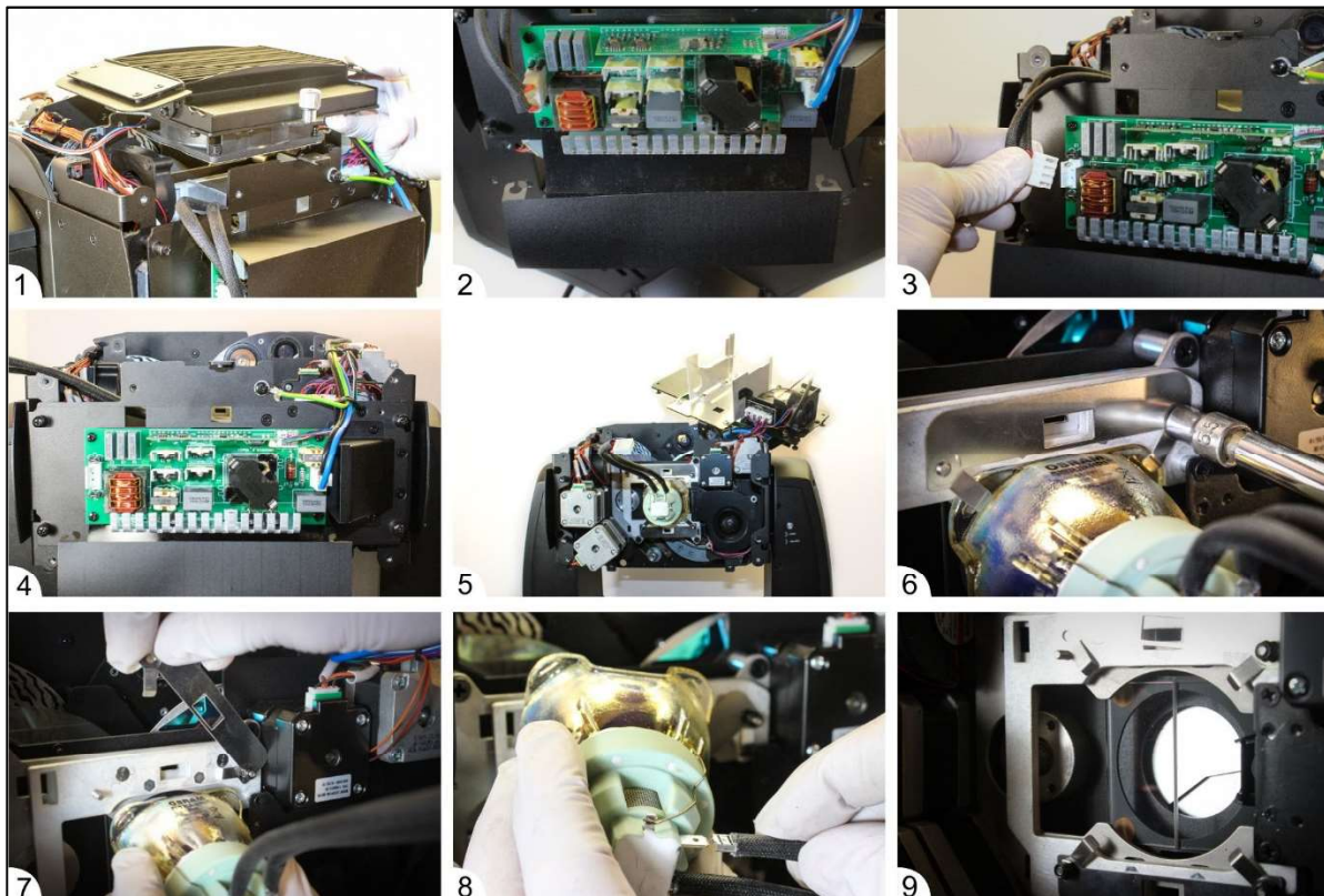
Figure 18. Lamp removal
